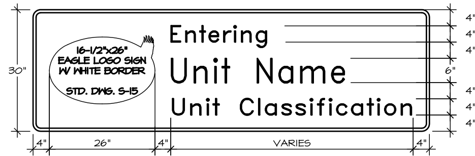
HIGHWAY GUIDE SIGN TYPE I-A
