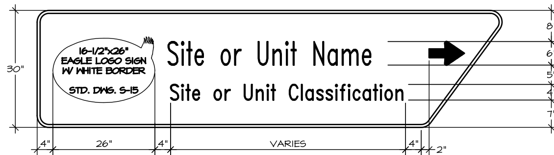
HIGHWAY GUIDE SIGN TYPE IIR
